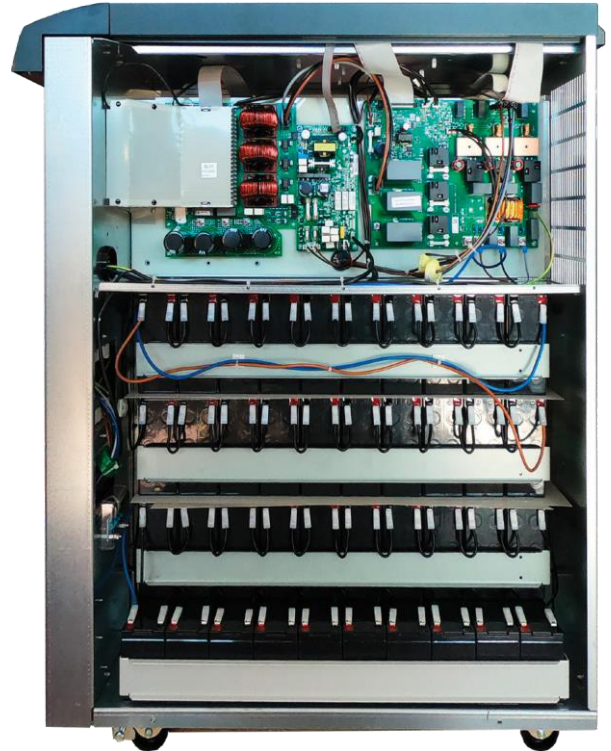
Roma (10-15-20KVA) with internal batteries installed
